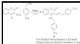
Fig. 1. Synthetic route for the title compound (I)
